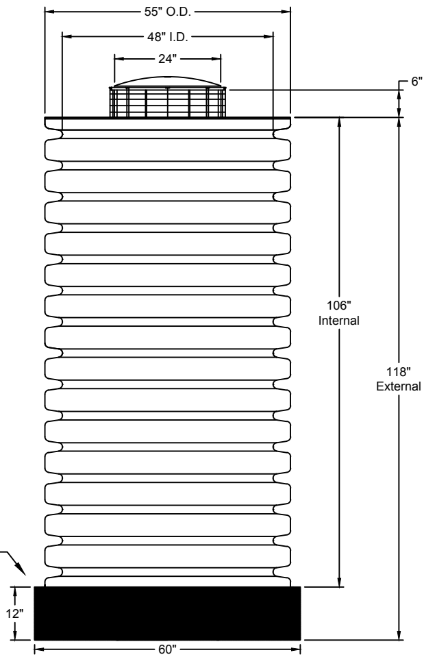
Side View
